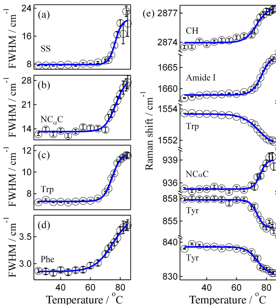
Figure 3. (a) Temperature-dependent FWHM of the Raman bands for SS stretching vibration, (b) N-C α -C stretching vibration, (c) benzene and pyrrole in-phase breathing vibration of Trp, and (d) benzene ring breathing vibration of Phe; (e) the temperature-dependent Raman shifts of the Raman bands for CH stretching vibration, amide I mode, C 2 =C 3 stretching vibration of Trp, N-C α -C stretching vibration, and the Fermi Resonance doublet of Tyr. The sigmoid function was employed to fit these data.
